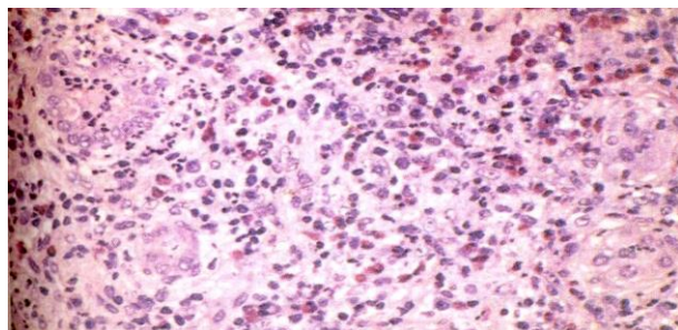
Figure No.3: Photomicrograph of 5 \mu\text{m} thick H&E stained paraffin section of rat kidney from group-C treated with diclofenac sodium, and vitamin-E, showing almost normal proximal convoluted tubules (PT) and distal convoluted tubules (DT) x416.
