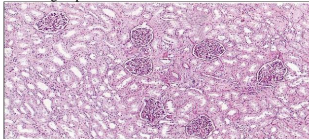
Figure No.1: Photomicrograph of 5 \mu\text{m} thick H&E stained paraffin section of rat kidney from group-A (control), showing normal architecture of renal cortex under low magnification. x101
