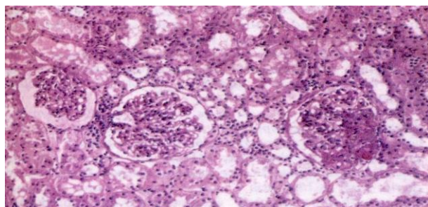
FigureNo.2:Photomicrograph of 5 \mu\text{m} thick H&E stained paraffin section of rat kidney from group-B treated with diclofenac sodium, showing dilated blood vessels with marked infiltration of inflammatory cells and damaged tubules. x205.
