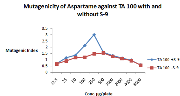
Figure No.3: Mutagenic potential of Aspartame against TA 100 with and without S-9
