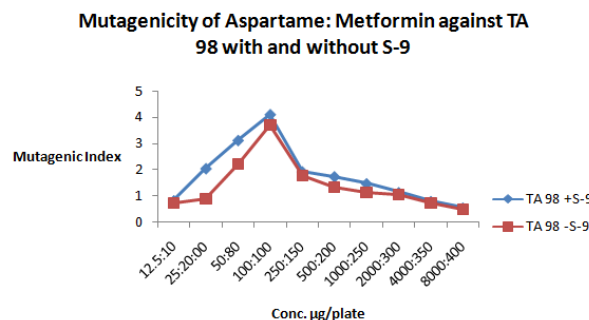
Figure No.6: Mutagenic Potential of ASP: MET against TA 98 with and without S-9
